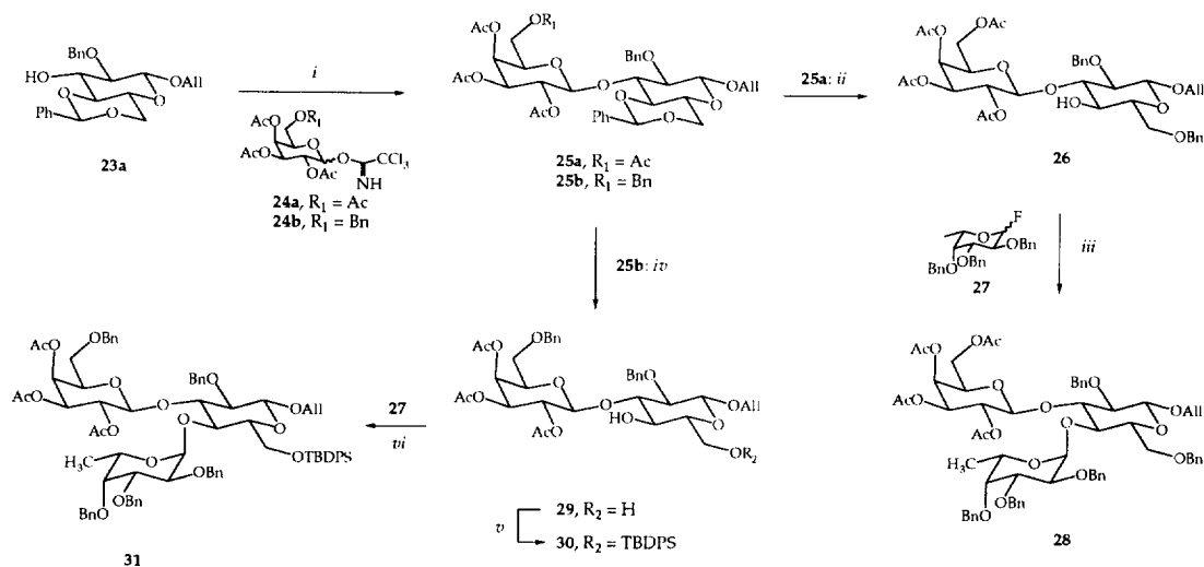
Scheme 3 a
