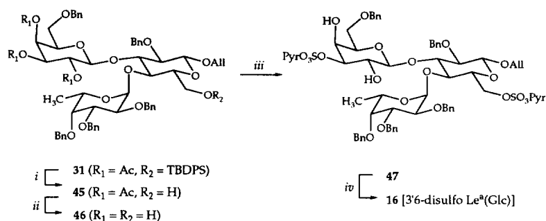
Scheme 8 a
