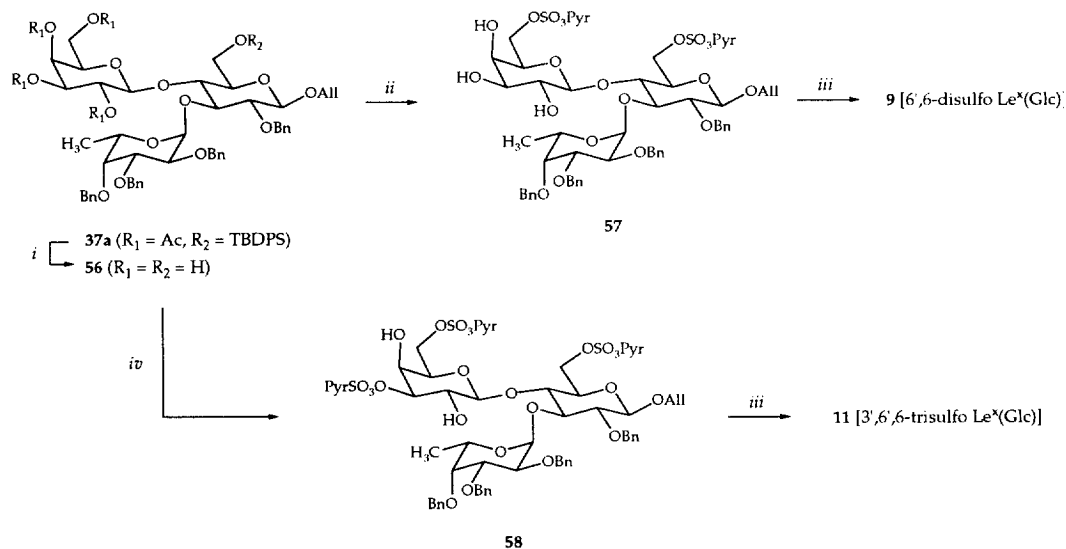
Scheme 11 a
