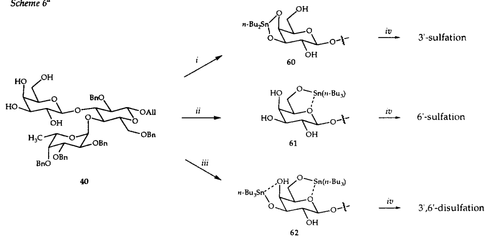
Scheme 6 a
