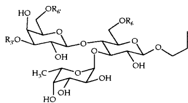
Sulfo Lewis x Derivatives
