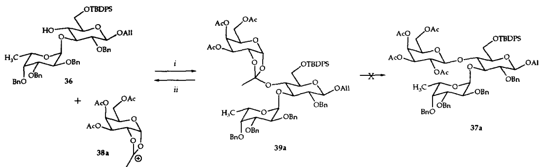
Scheme 5 a
