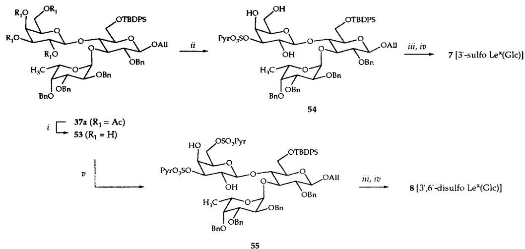
Scheme 10 a
