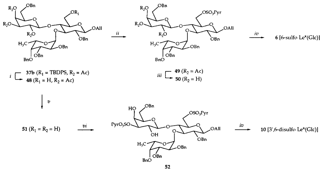
Scheme 9 a
