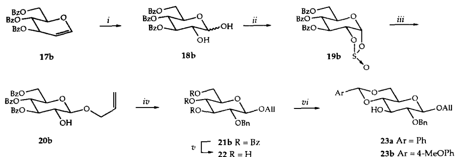
Scheme 2 a
