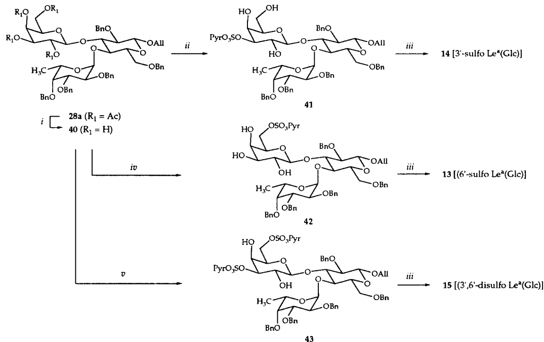
Scheme 7 a
