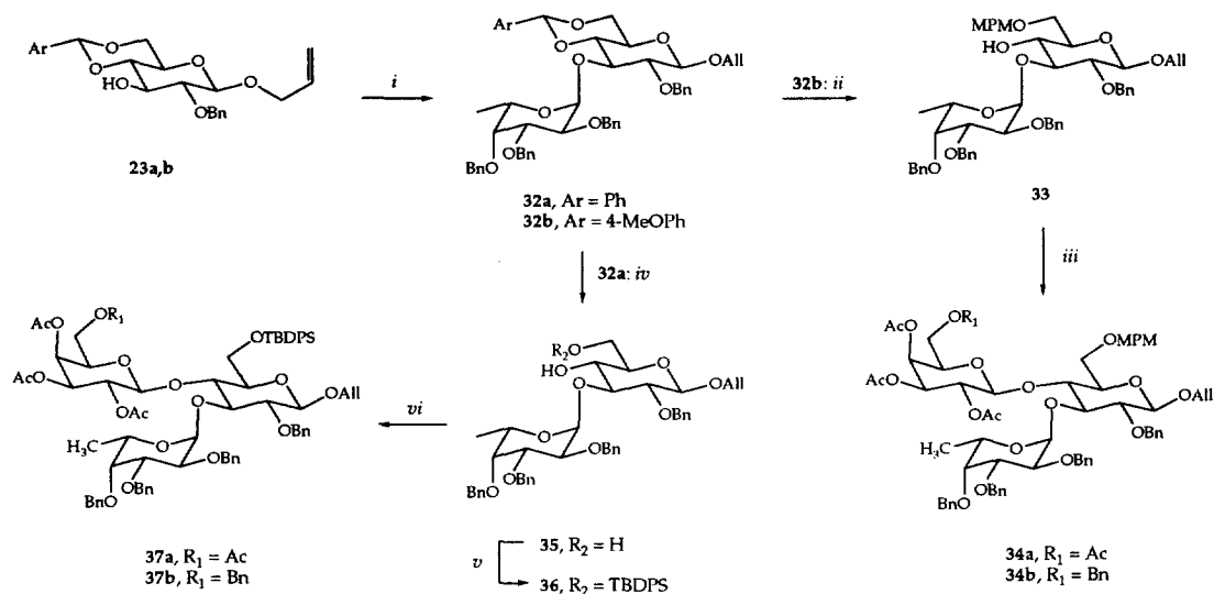
Scheme 4 a
