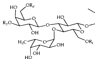
Sulfo Lewis a Derivatives
